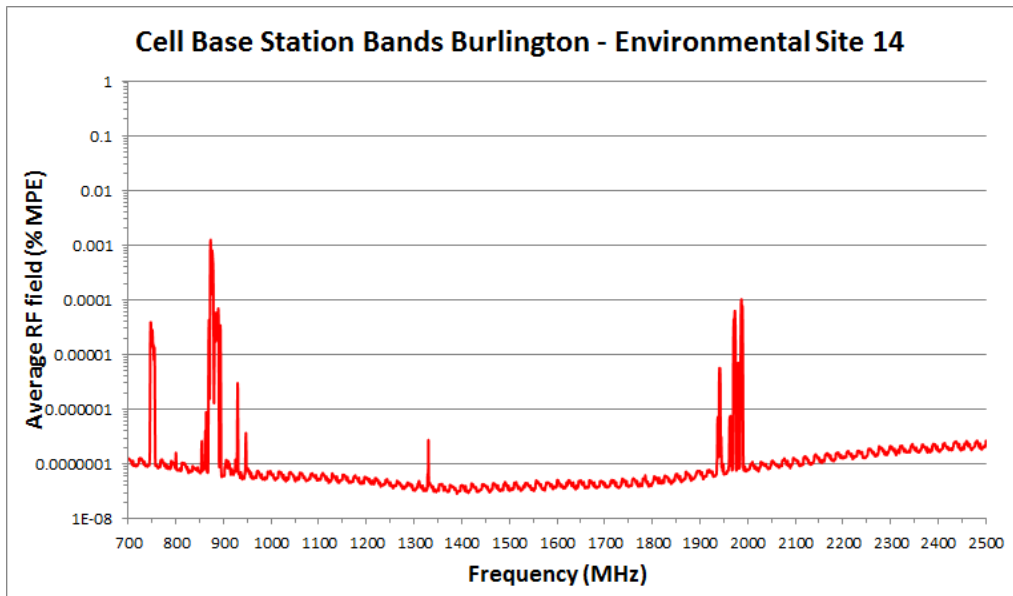
Figure 68. Spectrum measurement of average RF field (% MPE) across the wireless communication (cellular telephone) base station bands at environmental site 14 in Burlington.
