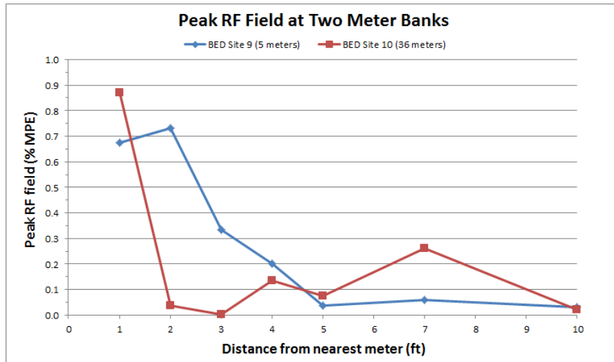
Figure 20. Measured peak RF fields of 900 MHz emissions observed at two meter banks (one with 5 meters and the other with 36 meters) in the BED service territory.
