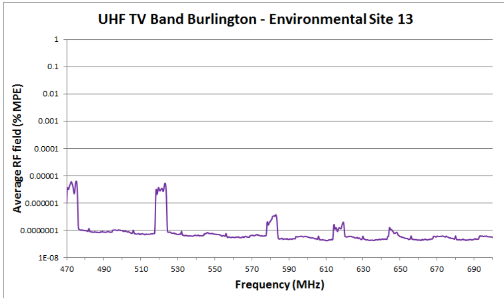
Figure 67. Spectrum measurement of average RF field (% MPE) across the UHF TV broadcast band at environmental site 13 in Burlington.
