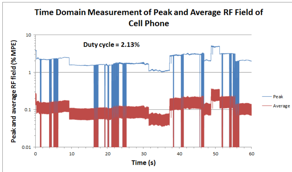
Figure 63. A measurement of the duty cycle of a cell phone across a 60 second phone call during which the phone was modulated with a moderate level of speech. The measured duty cycle was 2.13%.
