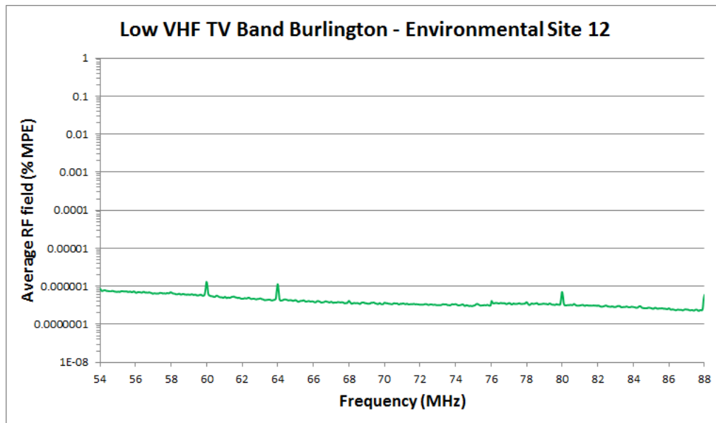
Figure 64. Spectrum measurement of average RF field (% MPE) across the low VHF TV broadcast band at environmental site 12 in Burlington.
