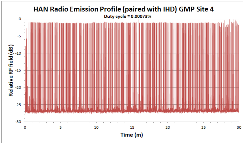
Figure 48. 30-minute HAN radio emission profile at GMP site 4 with radio paired to an IHD.
