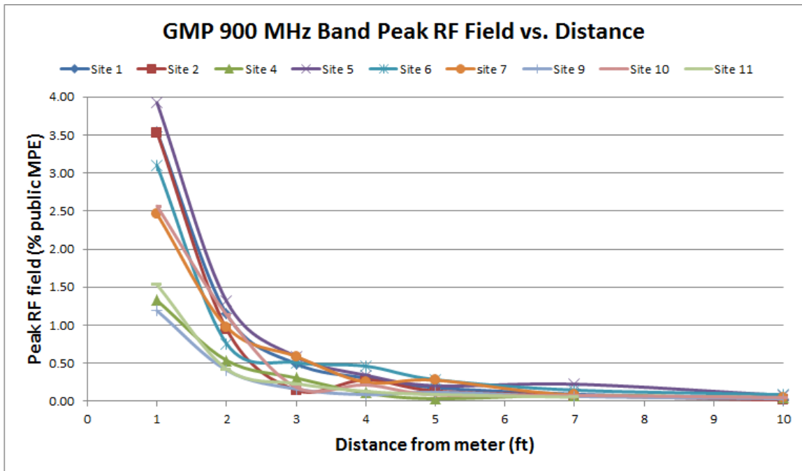
Figure 13. Linear display of measured peak values of RF fields at distances up to 10 feet in front of individual smart meters operated by GMP.
