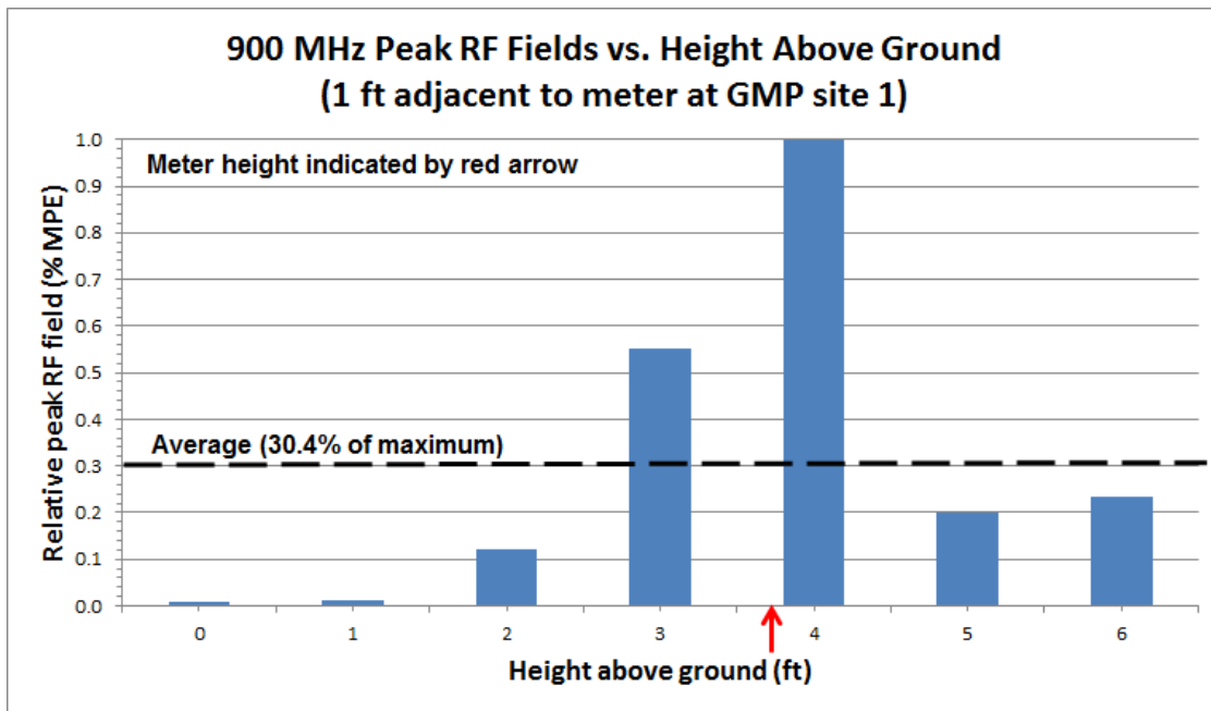
Figure 25. Relative peak RF field (as a percent of the MPE) vs. height above ground at one foot in front of a 900 MHz Elster meter operated by GMP in Vermont. Measured fields were normalized to the greatest value determined from all measurements. Overall, the spatial average was found to be 30.4% of the spatial maximum value. The variation in relative values is due to the fact that the smart meter emissions are mainly directed horizontal to the meter.
