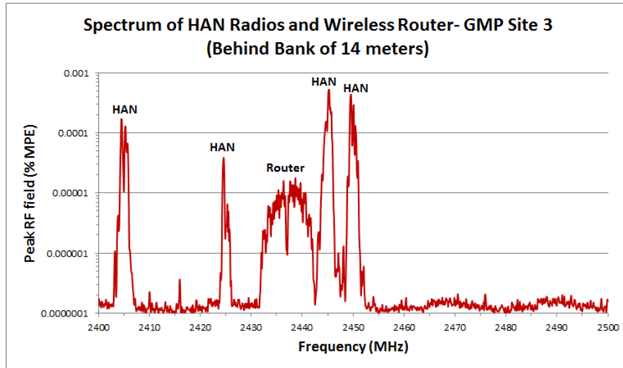
Figure 55. A measured spectrum of RF fields at GMP site 3, behind a bank of 14 smart meters, showing the presence of four HAN radio emissions and a wireless router.
